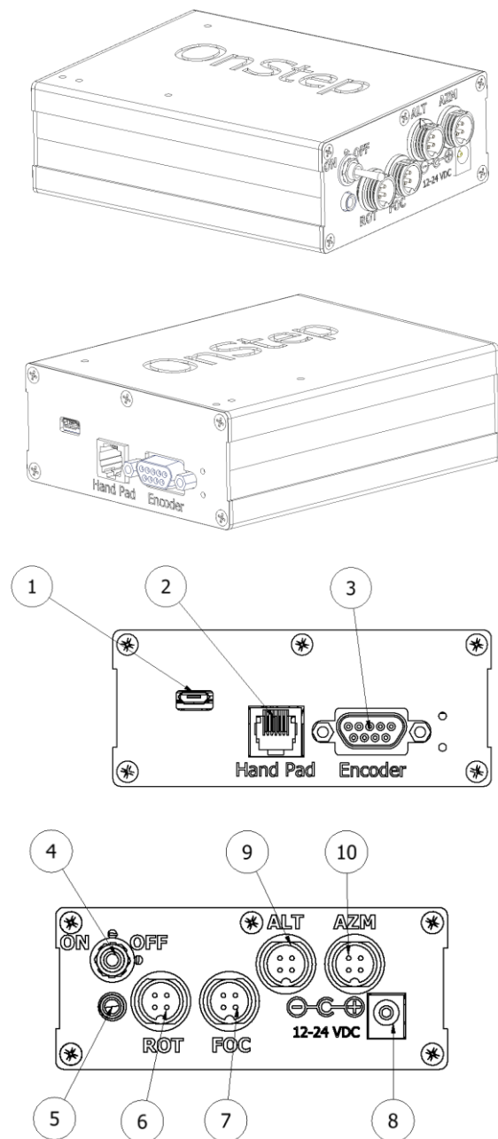
Goto Controller (UL12G-UL24G)
